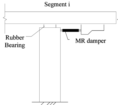
Fig. 2 MR damper between superstructure segment and the cap beam
