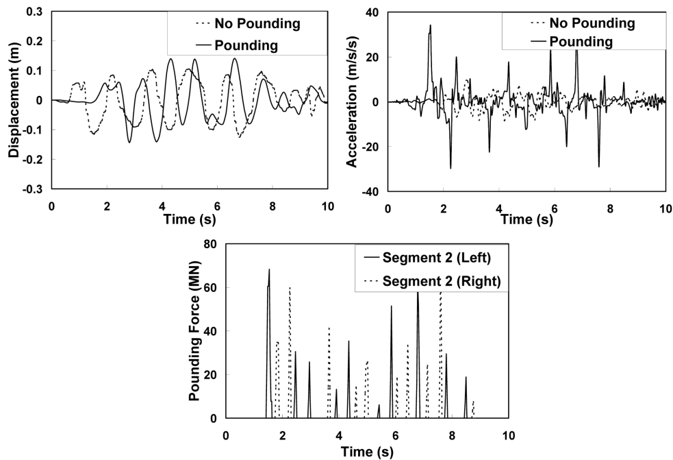
Fig. 5 Structural response of segment 2 under El Centro earthquake ground motion
