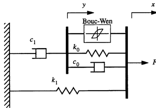
Fig. 3 Bouc-wen phenomenological model (Spencer et al. 2007)
