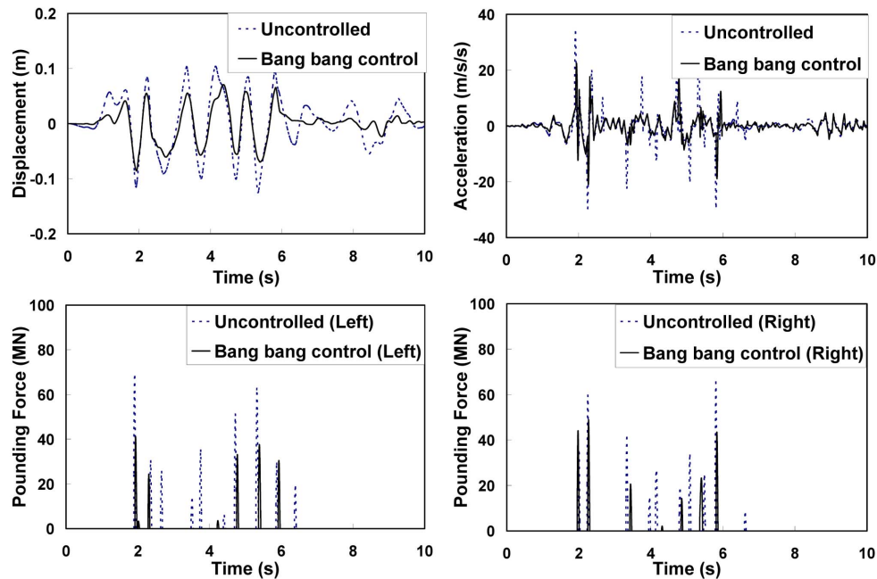
Fig. 8 Structural response of bridge (segment 2) with MR damper (bang bang control) under El Centro earthquake ground motion
