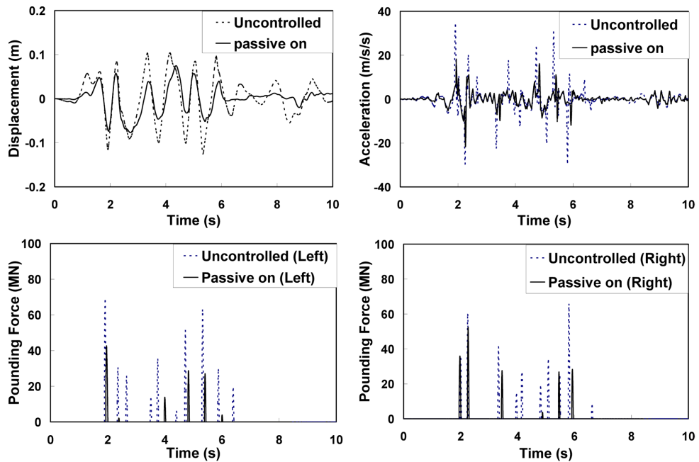
Fig. 7 Structural response of bridge (segment 2) with MR damper (passive on) under El Centro earthquake ground motion
