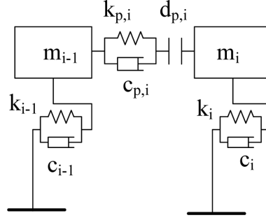
Fig. 1 Bridge pounding model based on contact element approach
