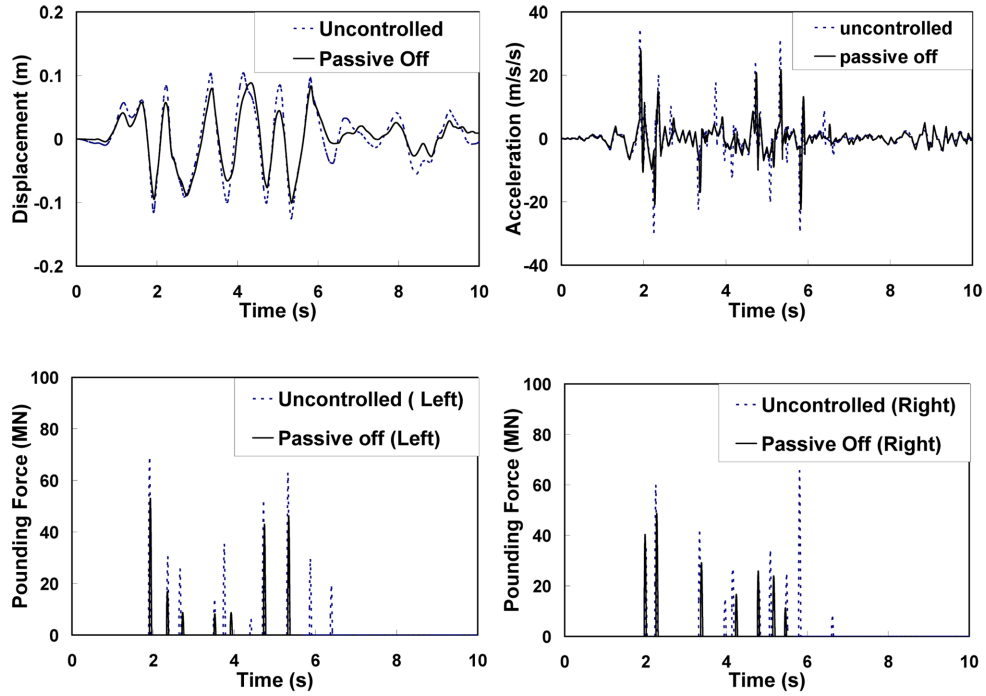
Fig. 6 Structural response of bridge (segment 2) with MR damper (passive off) under El Centro earthquake ground motion
