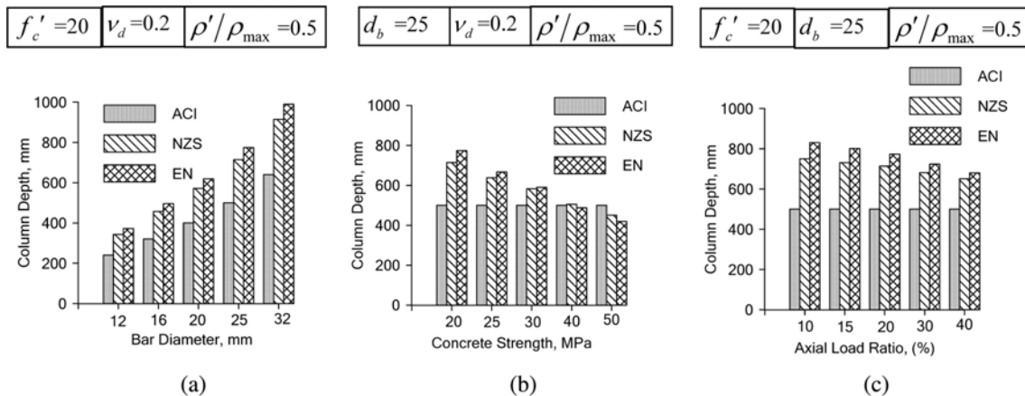
Fig. 3 Variation of column depth for interior joint
