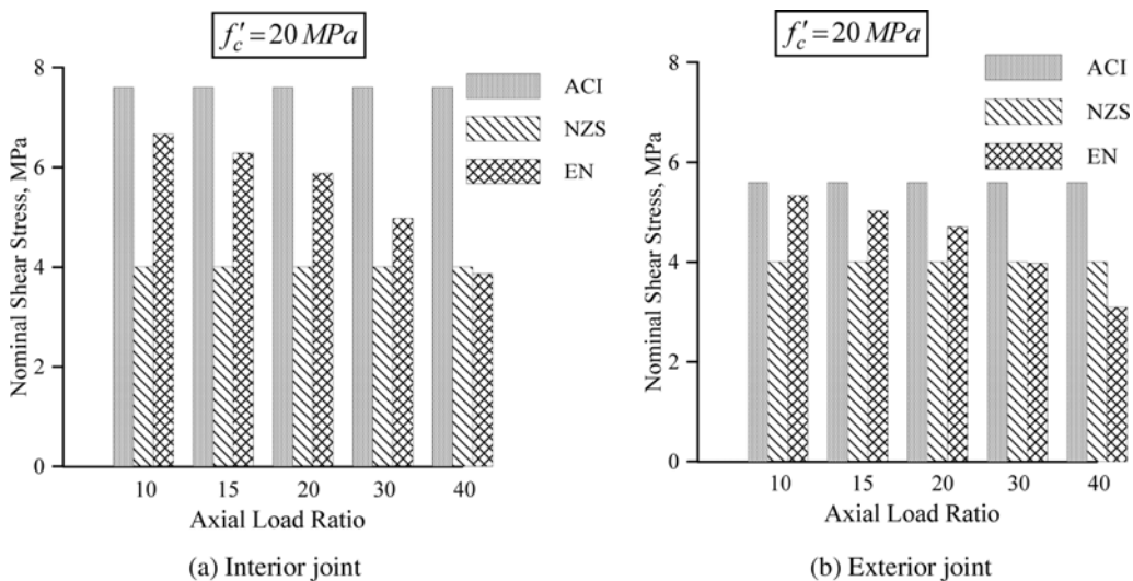
Fig. 8 Effect of axial load on nominal shear stress
