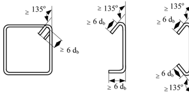
Fig. 11 Typical configurations of stirrup and cross-ties
