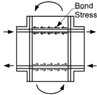
Fig. 2 Bond condition in an interior joint
