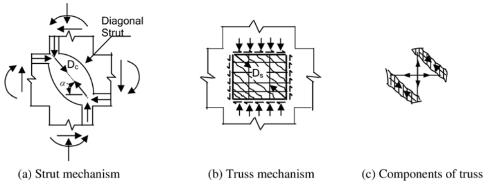
Fig. 6 Shear resisting mechanisms
