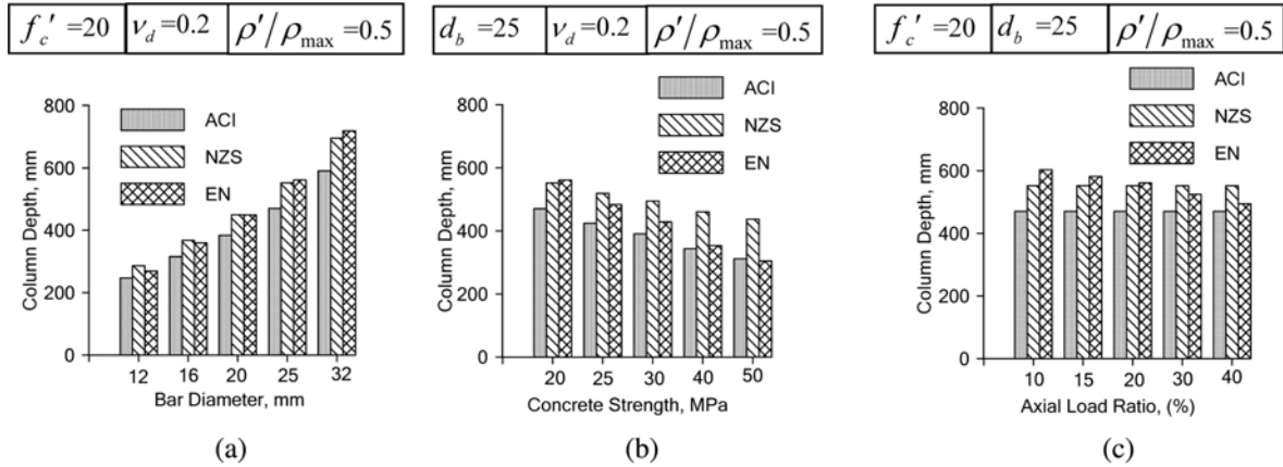
Fig. 5 Variation on column depth for exterior joint
