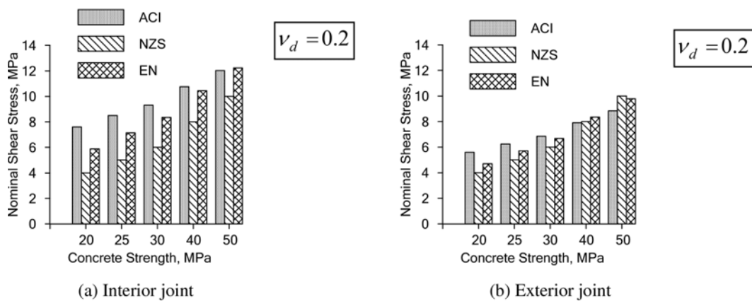
Fig. 7 Effect of concrete strength on nominal shear stress
