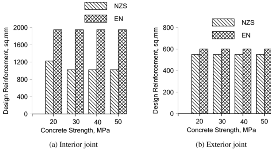
Fig. 10 Vertical design shear reinforcement
