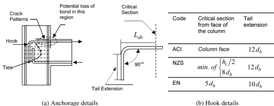
Fig. 4 Details of exterior joint
