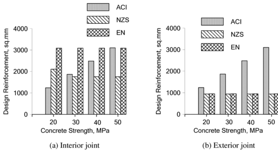
Fig. 9 Effect of concrete strength on design shear reinforcement
