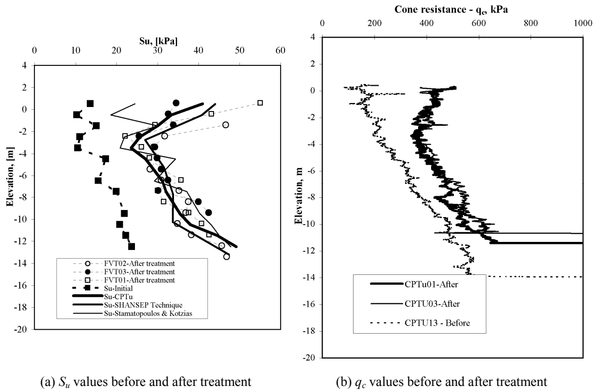
Fig. 10 Comparison S_u and q_c values before and after treatment
