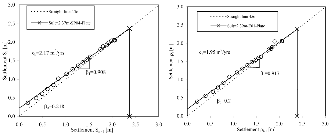
Fig. 11 Field settlement, Asaoka's plot for case study
