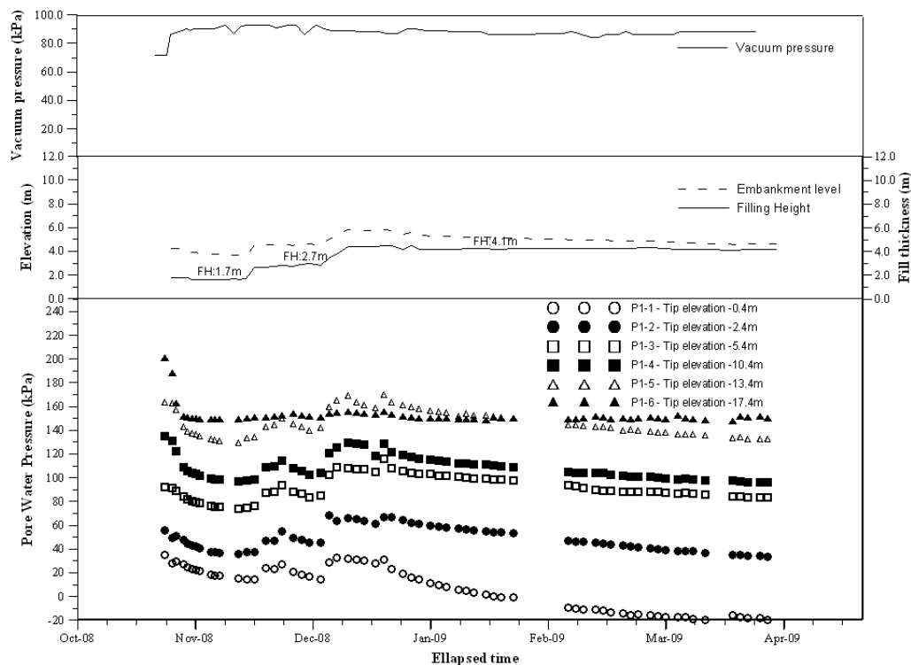
Fig. 6 Field pore-pressure measurements
