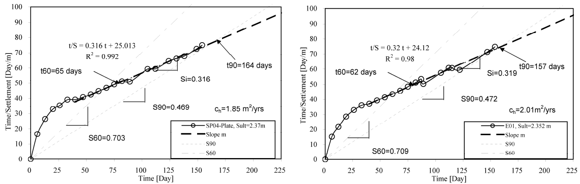
Fig. 12 Field settlement, hyperbolic's plot for case study
