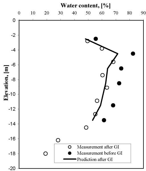
Fig. 9 Back-calculated water content from settlements
