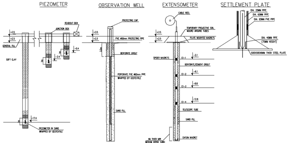
Fig. 4 Details of field instrumentations
