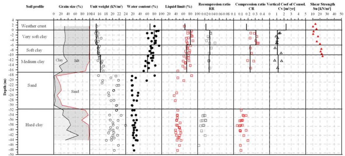
Fig. 2 Physical and mechanical properties of the subsoil at the testing site
