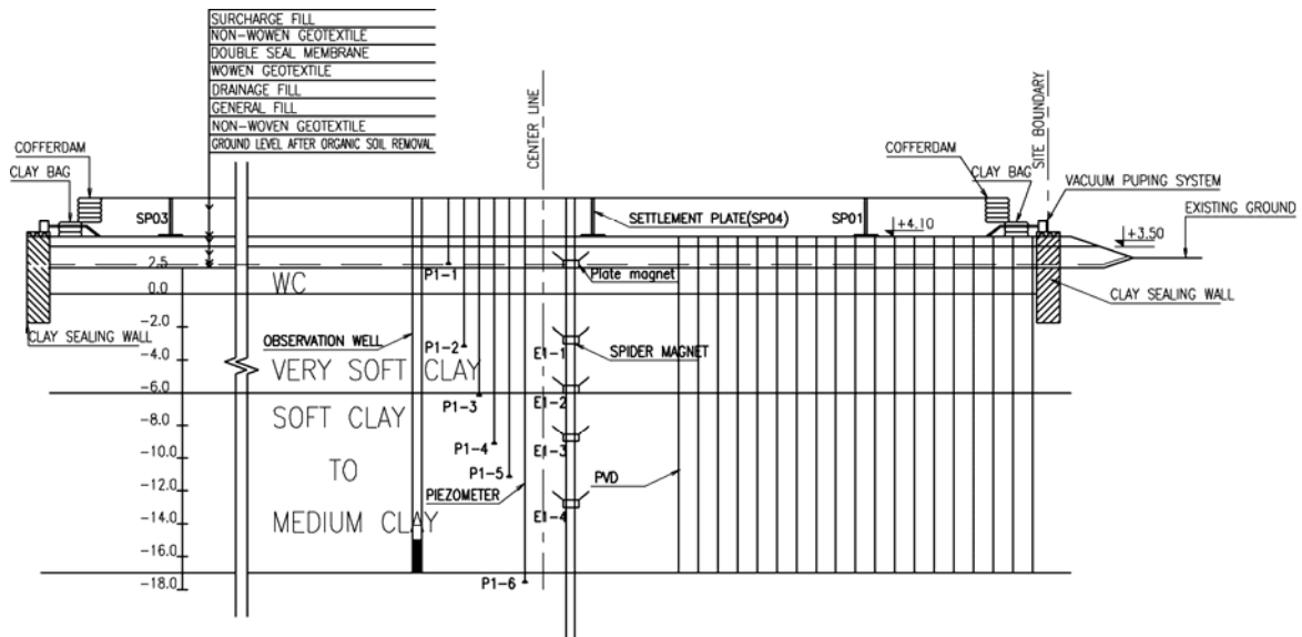
(a) Section A-A
