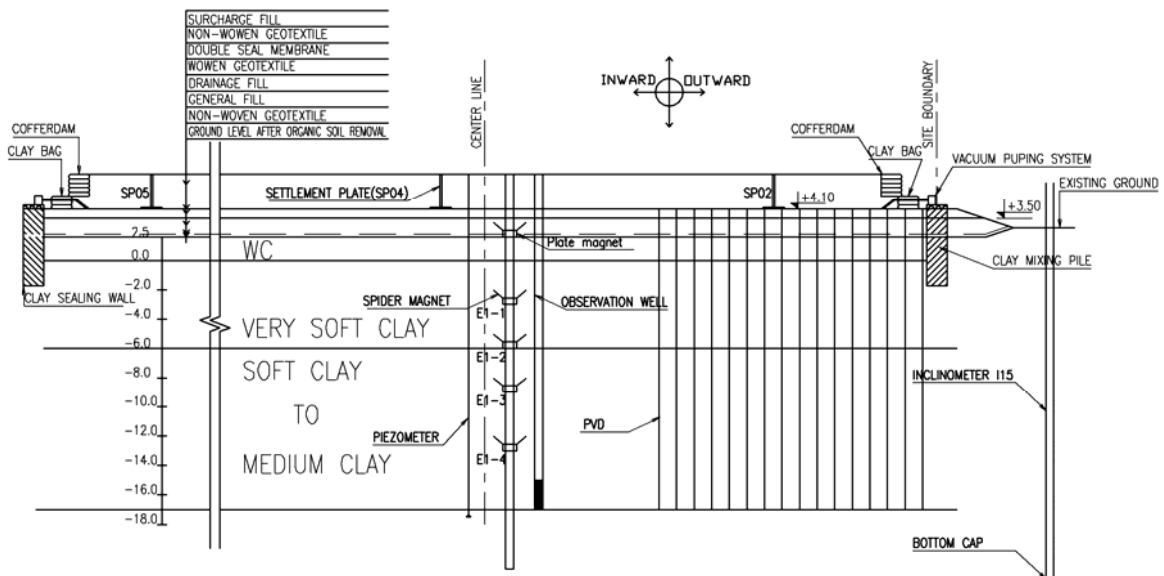
(b) Section B-B
