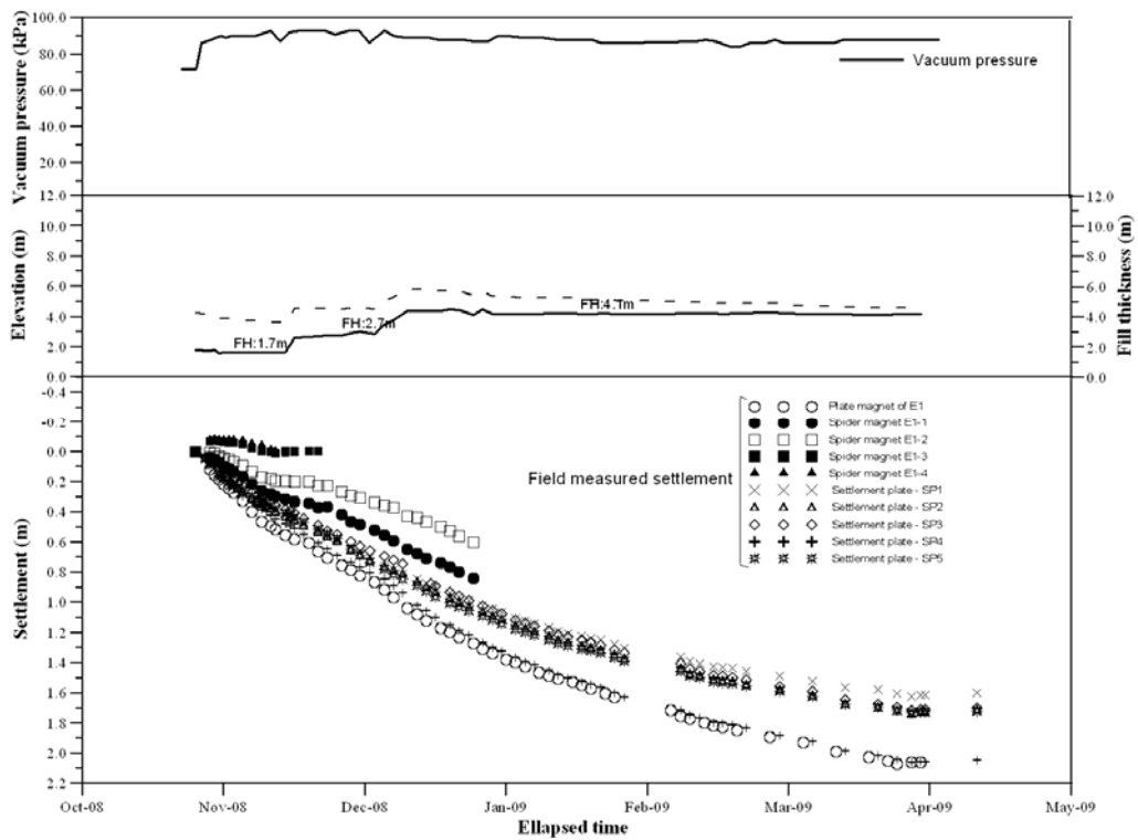
Fig. 5 Field settlement measurements
