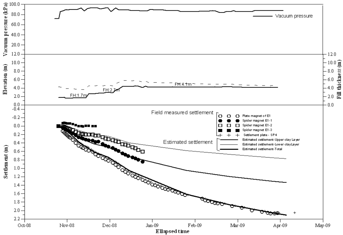
Fig. 8 Comparison of settlement between analytical results and monitoring data
