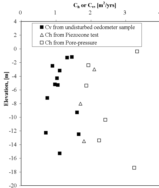
Fig. 13 Comparison of results of C_h from field measurements and C_v from oedometer test
