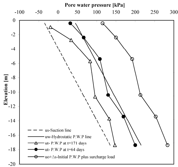
Fig. 7 Pore water pressure versus depths
