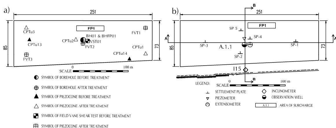
Fig. 1 (a) Locations of boreholes; and (b) Layout of installation of field instrumentations
