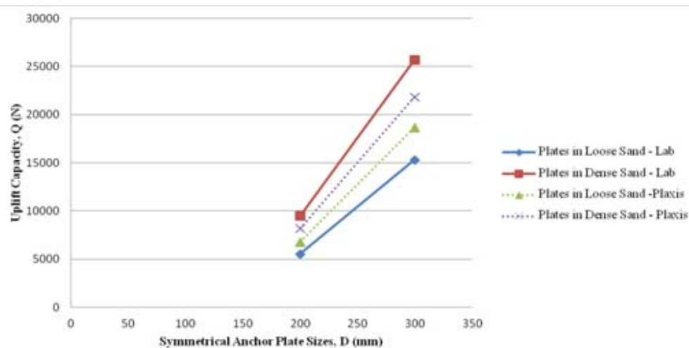
Fig. 8 Variation in uplift capacity Q with symmetrical anchor plate size D for rectangular anchor plate at L/D = 3 in loose and dense sand
