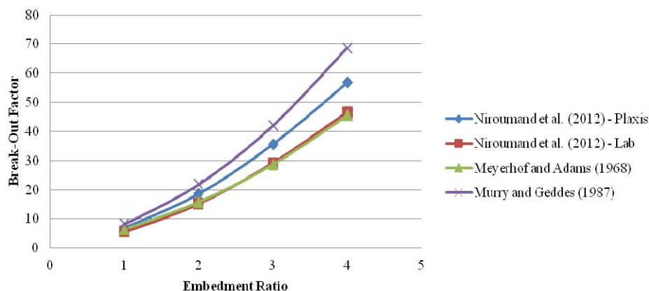
Fig. 11 Comparison of break-out factor between experimental results and theoretical and numerical prediction for rectangular anchor plates in loose packing
