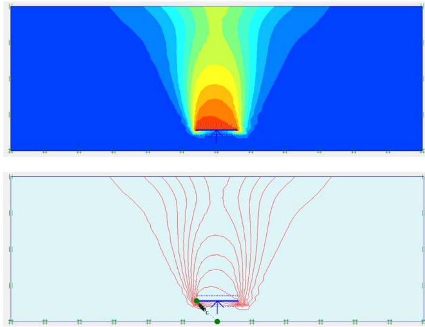
Fig. 14 State of sand after commencement of uplift in sand
