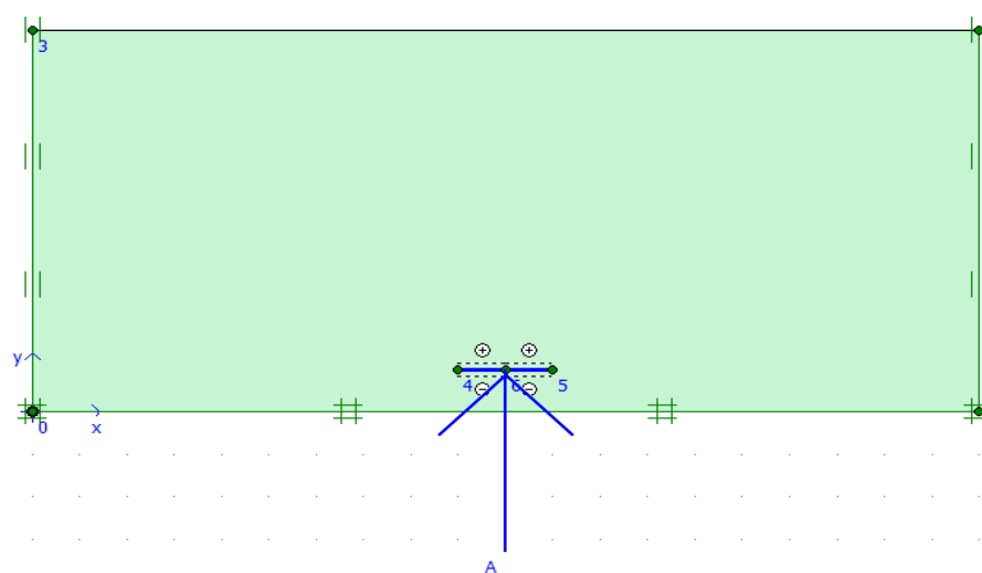
Fig. 7 The model geometry on prototype in Plaxis
