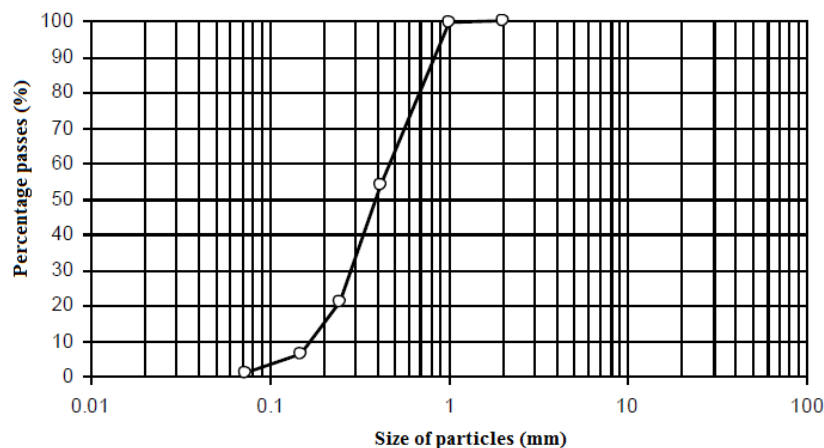
Fig. 3 Particle size distributions for sand sample
