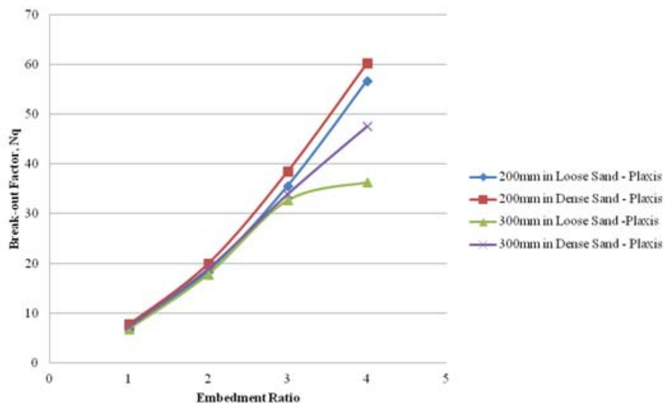
Fig. 10 Variation of break-out factor N_q with embedment ratio L/D for symmetrical rectangular anchor plates in both loose and dense packing in Plaxis
