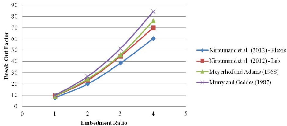
Fig. 11 Comparison of break-out factor between experimental results and theoretical and numerical prediction for rectangular anchor plates in dense packing
