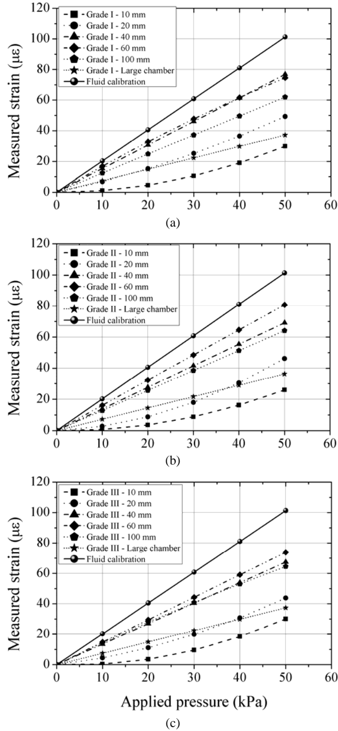
Fig. 8 Effect of sand bed thickness on performance of EPC: (a) Performance for sand of Grade I, (b) Performance for sand of Grade II and (c) Performance for sand of Grade III
