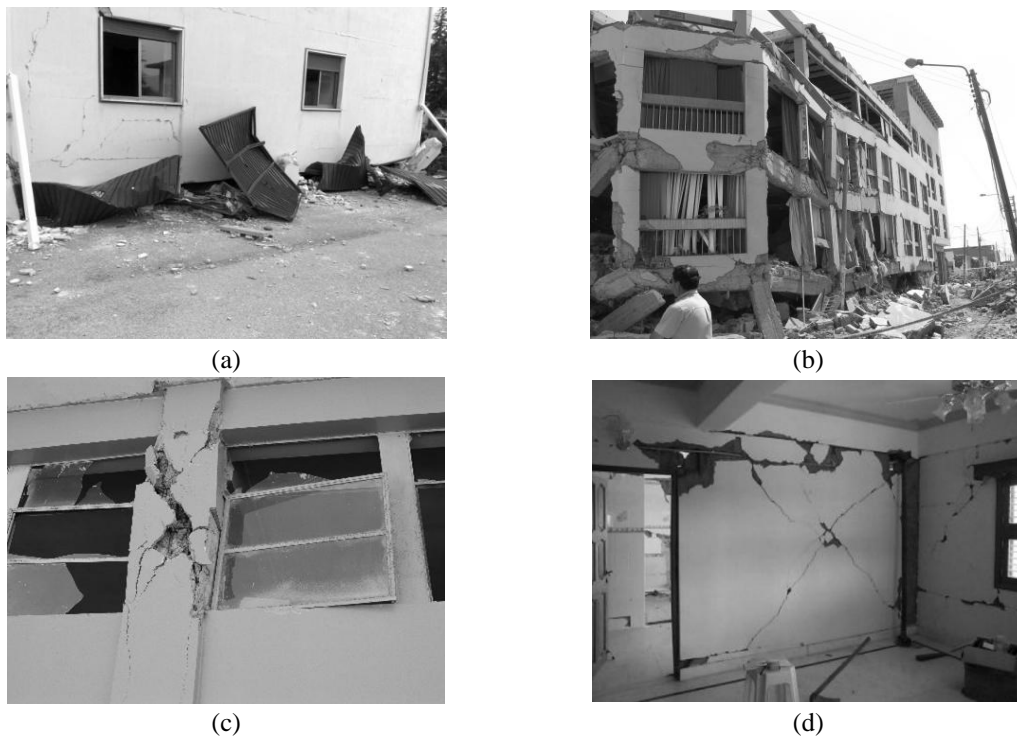
Fig. 3 Post-earthquake damage in infilled RC frames: soft-storey mechanism in (a) 2009 L'Aquila, Italy and (b) 2007 Pisco, Peru earthquakes; (c) short column effect in 2007 Pisco, Peru earthquake; (d) diagonal cracking at infill panels in 2001 Bhuj, India earthquake (Patel and Pindoria 2001)
