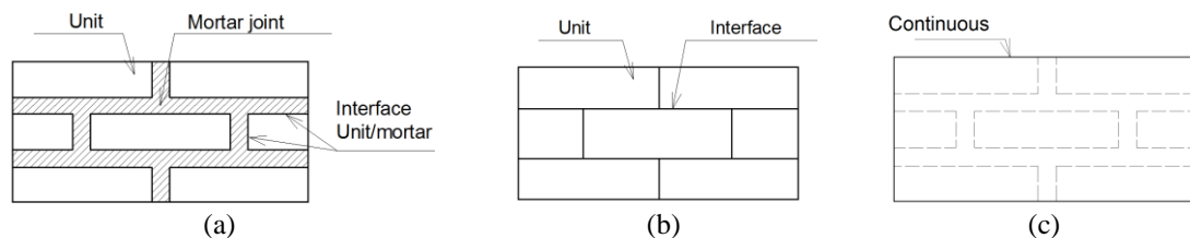
Fig. 10 Micro-model approach for the infill masonry panel; a) detailed micro-model; b) simplified micro-model with interface elements; c) meso-modelling
