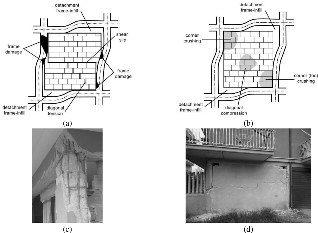
Fig. 2 Failure modes for infilled RC frames: (a) frame failure, sliding shear and diagonal cracking; (b) corner crushing and diagonal compression (adapted from Asteris et al. 2011); (c) example of frame failure; (d) example of sliding shear failure
