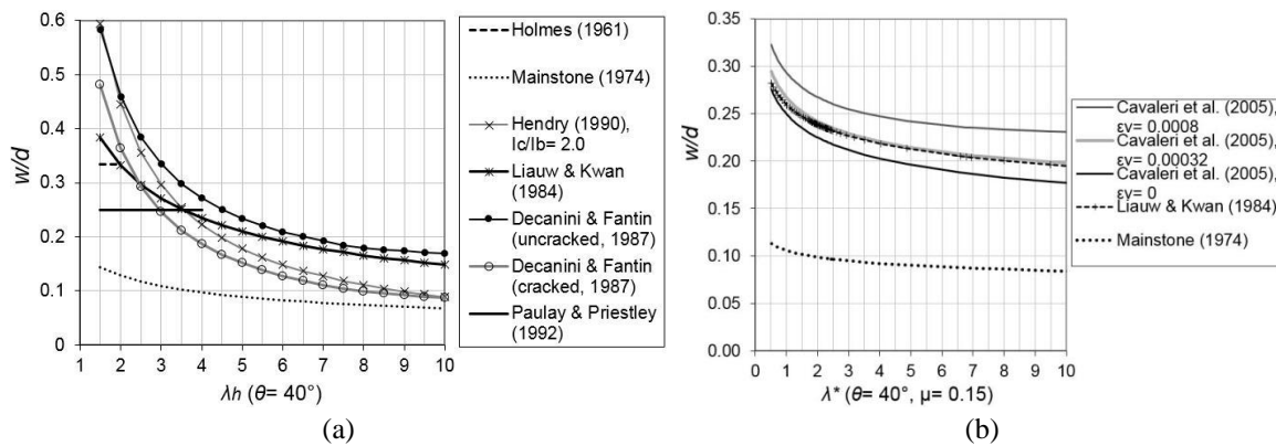
Fig. 7 Variation of the w/d ratio with respect to the relative stiffness (a) \lambda_h and (b) \lambda^*
