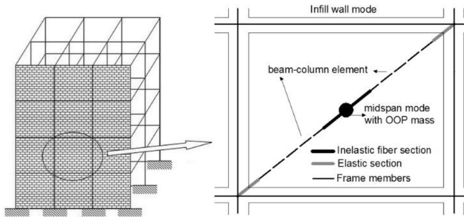
Fig. 6 Infill model by Kadysiewskil and Mosalam (2009), comprising a beam-column elements with fiber discretization (adapted from Kadysiewskil and Mosalam 2009)
