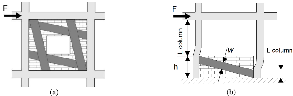
Fig. 4 (a) Typical strut-and-tie approach for panels with central openings and (b) for partially infilled frames (modified from Al-Chaar 2002)
