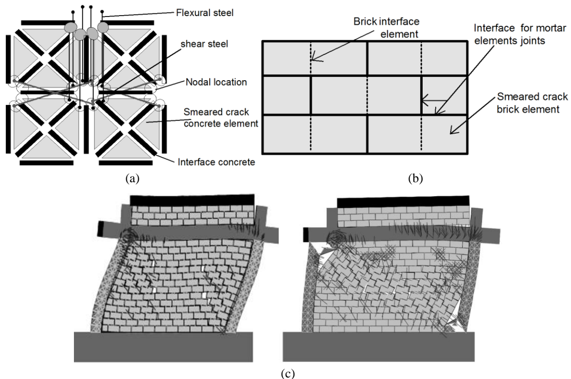
Fig. 12 Micro-model proposed by Stavridis and Shing (2010): (a) Finite element discretization of RC members; (b) finite element discretization of masonry infill (simplified micro-modelling); (c) numerical deformation and failure pattern of an infilled RC frame
