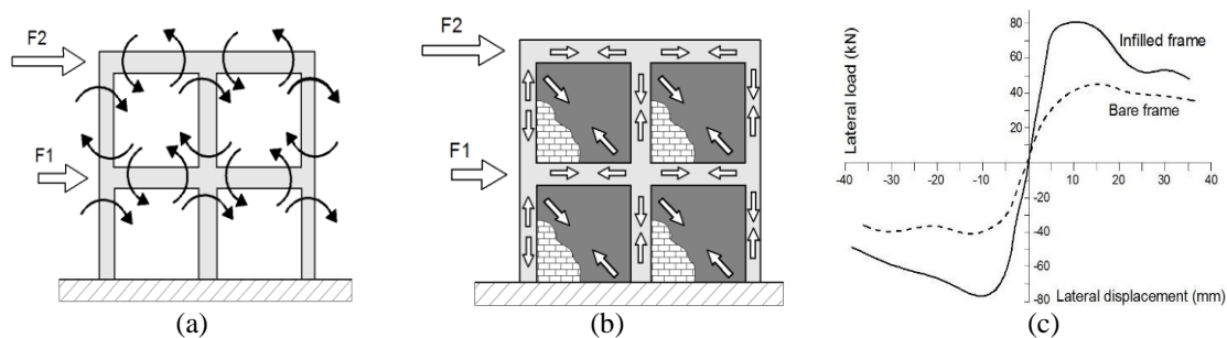
Fig. 1 Behaviour of frames under lateral loads: (a) bare frame, predominant frame action; (b) infilled frame, predominant truss action (adapted from Kaushik et al. 2006); (c) qualitative comparison of the experimental cyclic response of a RC frame with and without infill panels (adapted from Kakaletsis and Karayannis 2008)
