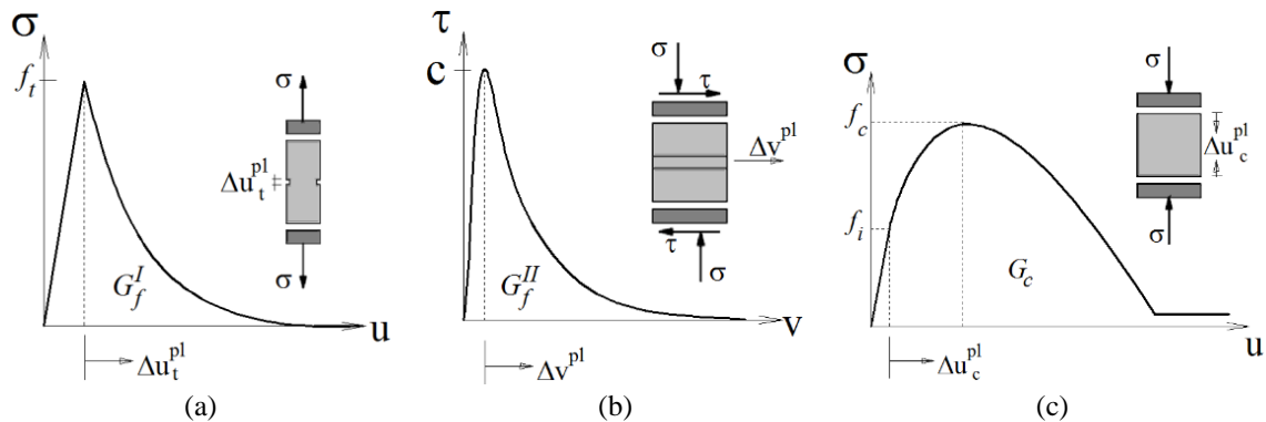
Fig. 11 Stress-displacement diagrams for quasi brittle materials, (a) tensile behaviour for mortar joints, (b) shear behaviour for mortar joints, (c) compressive behaviour of brick and mortar joints
