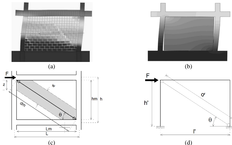
Fig. 5 Pushover finite element models for infill panels: (a) simplified micro model (adapted from Sattar 2013); (b) meso-modelling; (c) and (d) macro models, adapted from Crisafulli et al. 2000 and Amato et al. 2008, respectively
