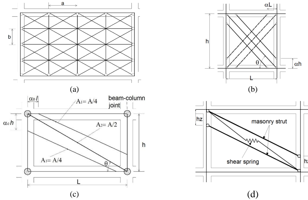
Fig. 8 Multiple equivalent (off-diagonal) strut models used by (a) Thiruvengadam (1985); (b) Chrysostomou et al. (2002), (Figure adapted from Asteris et al. 2011); (c) El-Dakhakhni et al. (2003); (d) Crisafulli and Carr (2007) - for simplicity, only struts in one direction are shown in (c) and (d)
