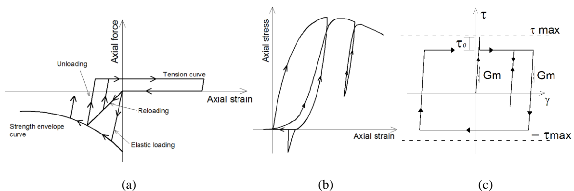
Fig. 9 Examples of hysteretic curves proposed for the equivalent struts representing masonry panels: (a) Klingner and Bertero (1978); (b) compression/tension and (c) shear cyclic response proposed by Crisafulli (1997)
