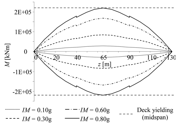
Fig. 13. Transverse bending moments for increasing values of IM for H/D = 9 and ground type A
